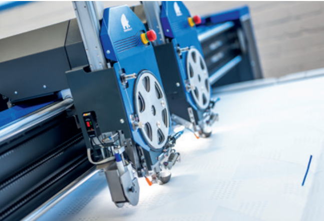
▲ Marking device for pattern-accurate cutting
