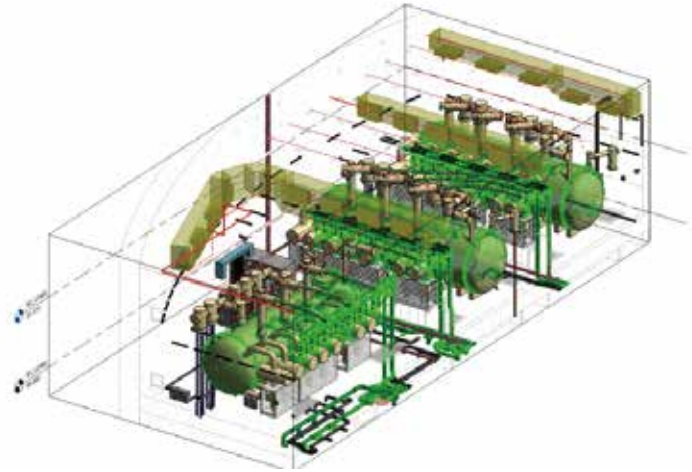
Underground 230kV GIT Substation, Singapore
