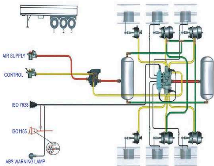
Anti Lock Braking System 4S/2M
