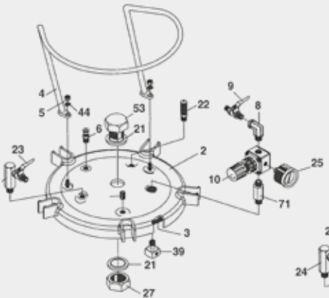
Model N: Version without PNEUMATIC AGITATOR
