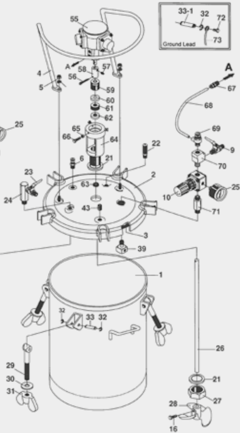
Model MN: Version with PNEUMATIC AGITATOR
