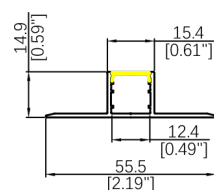
WL327A Length: 3.06M Diffuser: Silicone Down Light R>500mm Inward or Outward Light R>200mm
