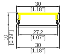
WL3010A Length: 3.06M Diffuser: Silicone Down Light R>300mm Inward or Outward Light R>150mm
