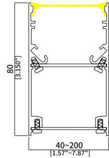
UGR080 Length: 2.8M Width: 40-200mm Optics: Diffuser/Prismatic + Diffuser Bend for Down Light R>40mm
