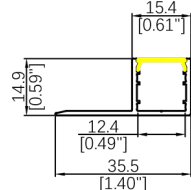
WL327B Length: 3.06M Diffuser: Silicone Down Light R>300mm
