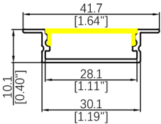
WL3010B Length: 3.06M Diffuser: Silicone Down Light R>300mm Inward or Outward Light R>150mm
