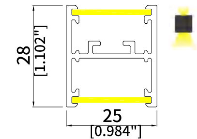
AR25 Length: 2.8M Diffuser: Silicone/PMMA Down Light R>180mm Inward or Outward Light R>150mm
