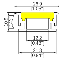
WL201 Length: 3.06M Diffuser: PP Down Light R>300mm
