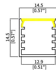
WL1515A Length: 3.06M Diffuser: Silicone Down Light R>180mm Inward or Outward Light R>150mm
