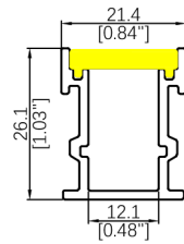
WL210 Length: 3.06M Diffuser: PP Down Light R>300mm
