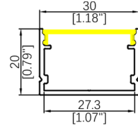
WL3020A Length: 3.06M Diffuser: Silicone Down Light R>300mm Inward or Outward Light R>200mm
