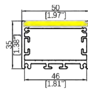
WL5035 Length: 3.3M Diffuser: Silicone/PP Down Light R>500mm
