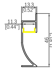
WL1346 Length: 1/2/3M Diffuser: Silicone Inward or Outward Light R>300mm
