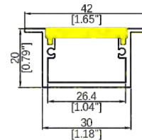
WL246A Length: 3.06M Diffuser: PP Down Light R>350mm
