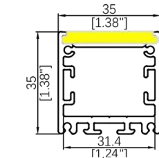
WL3535 Length: 2.9/3.3M Diffuser: Silicone/PP Down Light R>300mm Inward Light R>200mm
