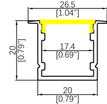
WL2020B Length: 3.06M Diffuser: Silicone Down Light R>150mm Inward or Outward Light R>120mm
