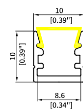
WL1010A Length: 3.06M Diffuser: Silicone Down Light R>180mm Inward or Outward Light R>150mm
