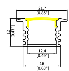
WL1612B Length: 3.06M Diffuser: Silicone Down Light R>180mm Inward or Outward Light R>150mm
