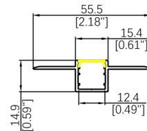
WL327 Length: 3.06M Diffuser: Silicone Down Light R>500mm Inward or Outward Light R>200mm
