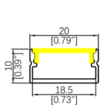
WL2010A Length: 3.06M Diffuser: Silicone Down Light R>180mm Inward or Outward Light R>150mm
