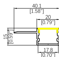
WL326C Length: 3.06M Diffuser: Silicone Down Light R>350mm
