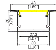
WL3020B Length: 3.06M Diffuser: Silicone Down Light R>400mm Inward or Outward Light R>200mm
