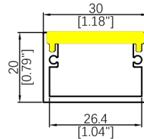
WL246 Length: 3.06M Diffuser: PP Down Light R>300mm
