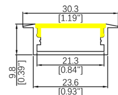
WL2410B Length: 3.06M Diffuser: Silicone Down Light R>300mm Inward or Outward Light R>150mm
