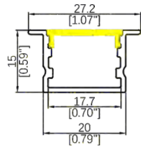
WL2015B Length: 3.06M Diffuser: Silicone Down Light R>180mm Inward or Outward Light R>150mm
