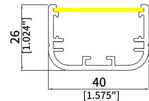
AR40 Length: 2.8M Diffuser: Silicone/PMMA Down Light R>180mm Inward or Outward Light R>150mm
