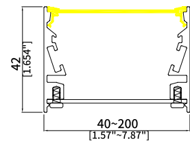
UGR042 Length: 2.8M Width: 40-200mm Optics: Diffuser/Prismatic + Diffuser Bend for Down Light R>40mm
