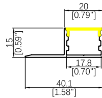
WL326B Length: 3.06M Diffuser: Silicone Down Light R>450mm
