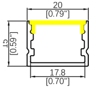
WL2015A Length: 3.06M Diffuser: Silicone Down Light R>180mm Inward or Outward Light R>150mm
