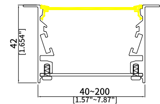
UGR042B Length: 2.8M Width: 40-200mm Optics: Diffuser/Prismatic + Diffuser Bend for Down Light R>40mm
