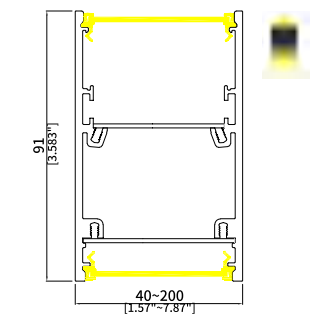
AM091 Length: 2.8M Width: 40-200mm Optics: Diffuser/Prismatic + Diffuser Bend for Down Light R>40mm
