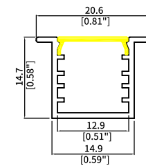
WL1515B Length: 3.06M Diffuser: Silicone Down Light R>180mm Inward or Outward Light R>150mm
