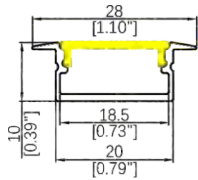
WL2010B Length: 3.06M Diffuser: Silicone Down Light R>180mm Inward or Outward Light R>150mm
