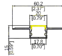
WL326 Length: 3.06M Diffuser: Silicone Down Light R>700mm Inward or Outward Light R>300mm
