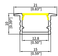
WL1510B Length: 3.06M Diffuser: Silicone Down Light R>180mm Inward or Outward Light R>150mm
