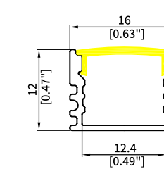
WL1612A Length: 3.06M Diffuser: Silicone Down Light R>180mm Inward or Outward Light R>150mm
