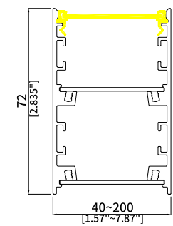
UGR072 Length: 2.8M Width: 40-200mm Optics: Diffuser/Prismatic + Diffuser/Optics Bend for Down Light R>40mm
