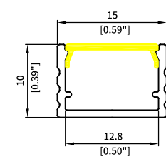
WL1510A Length: 3.06M Diffuser: Silicone Down Light R>180mm Inward or Outward Light R>150mm
