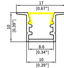
WL1010B Length: 3.06M Diffuser: Silicone Down Light R>180mm Inward or Outward Light R>150mm
