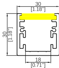
WL3030 Length: 2.9/3.6/4.1M Diffuser: Silicone/PP Down Light R>260mm Inward Light R>150mm
