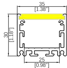
WL3530 Length: 3.3M Diffuser: Silicone/PP Down Light R>300mm Inward Light R>200mm
