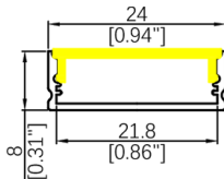
WL2410A Length: 3.06M Diffuser: Silicone Down Light R>300mm Inward or Outward Light R>150mm
