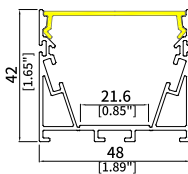
UGR4842 Size: W48xH42mm Housing: Matt Black/White PCB Width: 20mm
