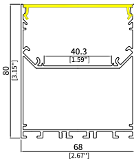
UGR6880 Size: W68xH80mm Housing: Matt Black/White PCB Width: 40mm
