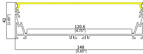
UGR14842 Size: W148xH42mm Housing: Matt Black/White PCB Width: 120mm
