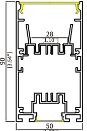
CS5090S Size: W50xH90mm Housing: Anodized Silver/ Matt Black/ Matt White PCB Width: 28mm Endcap: Aluminum
