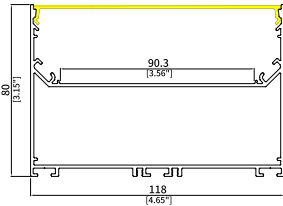
UGR11880 Size: W118xH80mm Housing: Matt Black/White PCB Width: 90mm
