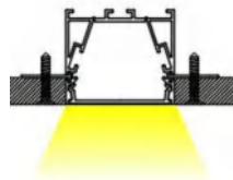
R1 Trimless Recessed for plaster
