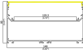
UGR14880 Size: W148xH80mm Housing: Matt Black/White PCB Width: 120mm
