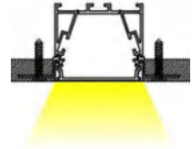
R2 Trimless Recessed for gypsum board
