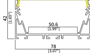
UGR7842 Size: W78xH42mm Housing: Matt Black/White PCB Width: 50mm
