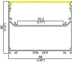
UGR9880 Size: W98xH80mm Housing: Matt Black/White PCB Width: 70mm
