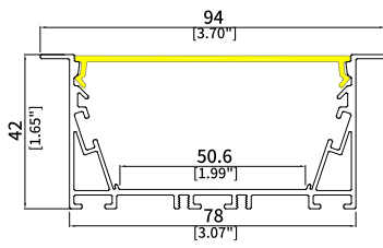
UGR7842B Size: W94xH42mm Cutout: 78mm Housing: Matt Black/White PCB Width: 50mm
