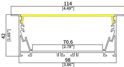
UGR9842B Size: W114xH42mm Cutout: 98mm Housing: Matt Black/White PCB Width: 70mm
