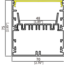
CS7075T Size: W70xH75mm Housing: Anodized Silver/ Matt Black/ Matt White PCB Width: 48mm Endcap: Aluminum
