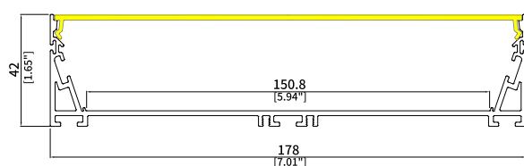
UGR17842 Size: W178xH42mm Housing: Matt Black/White PCB Width: 150mm
