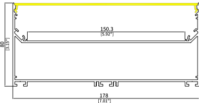
UGR17880 Size: W178xH80mm Housing: Matt Black/White PCB Width: 150mm
