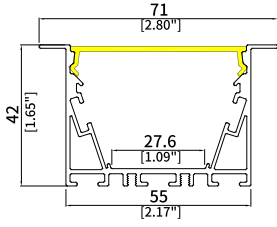
UGR5542B Size: W71xH42mm Cutout: 55mm Housing: Matt Black/White PCB Width: 27mm
