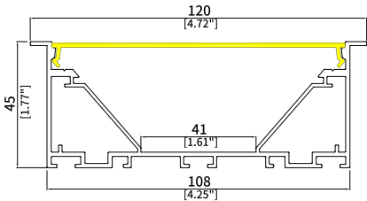
UGR120A Size: W120xH45mm Cutout: 108mm Housing: Matt Black/White PCB Width: 41mm
