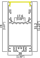
UGR3878 Size: W38xH78mm Housing: Matt Black/White PCB Width: 17mm
