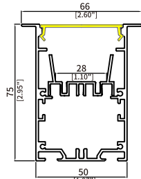
CS5075A Size: W66xH75mm Cutout: 50mm Housing: Anodized Silver/ Matt Black/ Matt White PCB Width: 28mm Endcap: Aluminum
