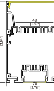
CS7090S Size: W70xH100mm Housing: Anodized Silver/ Matt Black/ Matt White PCB Width: 48mm Endcap: Aluminum
