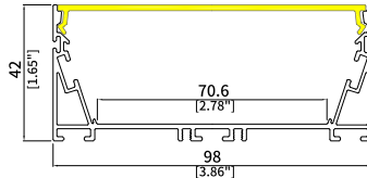
UGR9842 Size: W98xH42mm Housing: Matt Black/White PCB Width: 70mm
