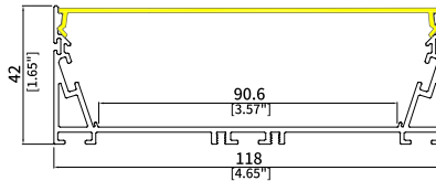
UGR11842 Size: W118xH42mm Housing: Matt Black/White PCB Width: 90mm
