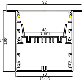
CS7075A Size: W92xH75mm Cutout: 70mm Housing: Anodized Silver/ Matt Black/ Matt White PCB Width: 48mm Endcap: Aluminum
