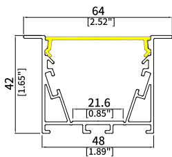
UGR4842B Size: W64xH42mm Cutout: 48mm Housing: Matt Black/White PCB Width: 21mm
