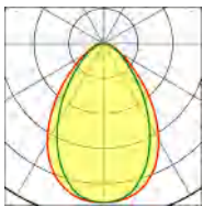
Clear Microprismatic Lens+ Linear Prism Sheet ~65°+ 80° Medium Beam
