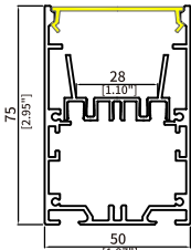
CS5075T Size: W50xH75mm Housing: Anodized Silver/ Matt Black/ Matt White PCB Width: 28mm Endcap: Aluminum
