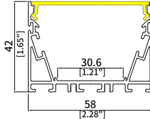
UGR5842 Size: W58xH42mm Housing: Matt Black/White PCB Width: 30mm
