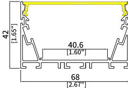
UGR6842 Size: W68xH42mm Housing: Matt Black/White PCB Width: 40mm
