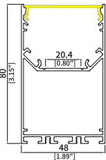
UGR4880 Size: W48xH80mm Housing: Matt Black/White PCB Width: 20mm
