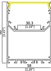
UGR5880 Size: W58xH80mm Housing: Matt Black/White PCB Width: 30mm
