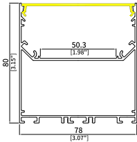
UGR7880 Size: W78xH80mm Housing: Matt Black/White PCB Width: 50mm
