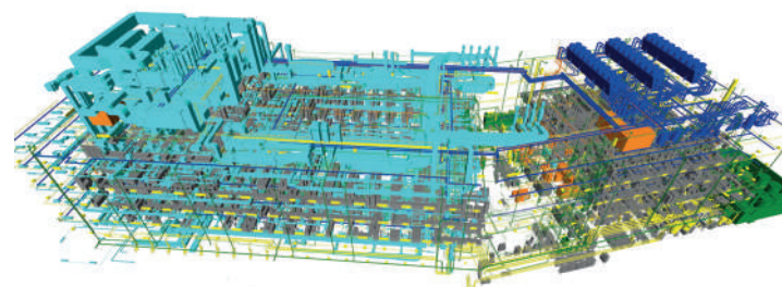
BIM MODEL
