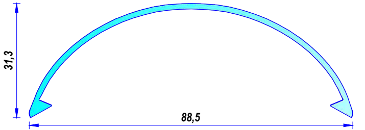
YA-P01 A PC. Diffuser Opal - Transparent
