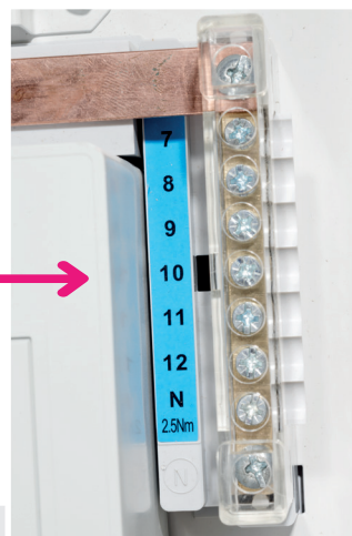
Shrouded Neutral Terminals
