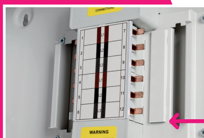
Robust pan assembly with device end stops
