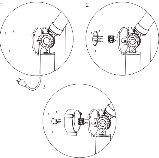
Drawings of the installation options of the Mr. Tubes LED driver separate: available on request or check tonone.com .
