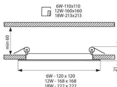
GRID LED 6W BK
