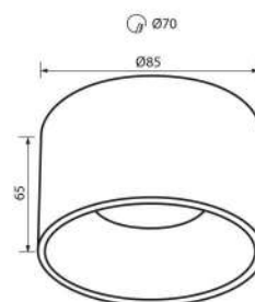
SL513 BK/G POLLA
