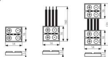
CONNECTORS RGB 10 mm
