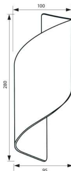
APOLLO LED BK/G
