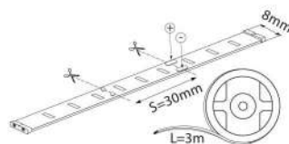
L=3m=30*100mm=90LED RGB BAGRA LED 30 SMD5050 - 3m SET
