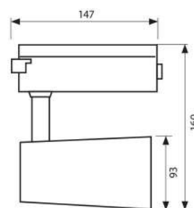
CLUB LED 20W/WH
