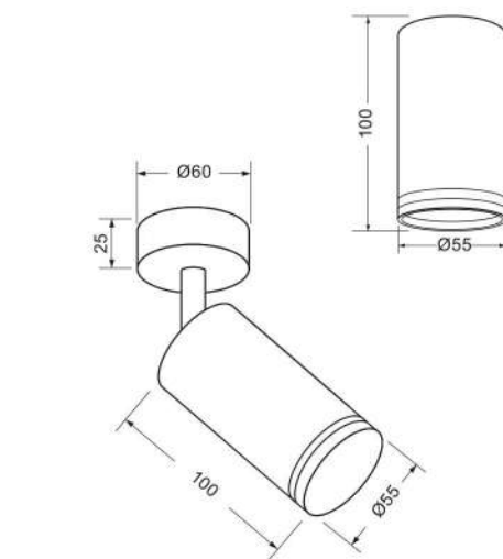
DL715 WH KING
