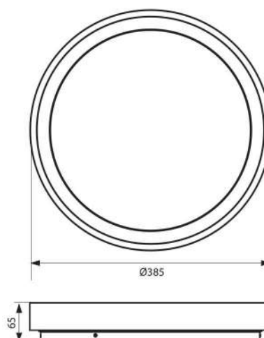
PLEADA LED RGB
