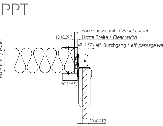
Abb. 4.4 U-Klemmrahmen Fig. 4.4 U-Clamping frame
