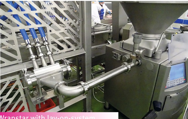
Wrapstar with lay-on-system
