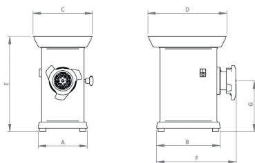
P-22. Production \pm 300 kg/h. Motor Power 1.5HP. P-32. Production \pm 425 kg/h. Motor Power 2.5HP.
