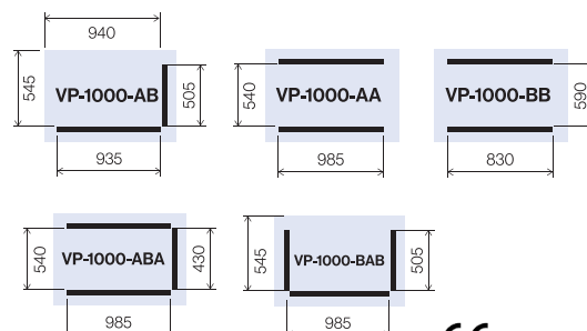
VP-1000 High lid AB; AA; BB, ABA, BAB HIGH. BUSCH pump 100m³/h.
