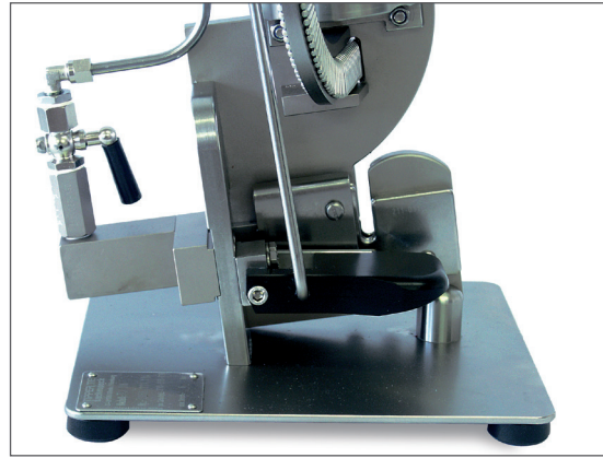
Triggering by a sensor lever and disengageable cutting knife.
