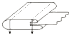
F8764 橫筒褲頭筒(環底) Right Angle Waist Band Folder (Close Bottom)
