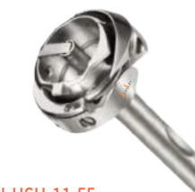
KLH-HSH-11-55 HSH-11-55 KRT11-5 JUKI LU-53 LU-562 SEIKO STW-6 8B 8BV 8V SINGER 111W155 211W155
