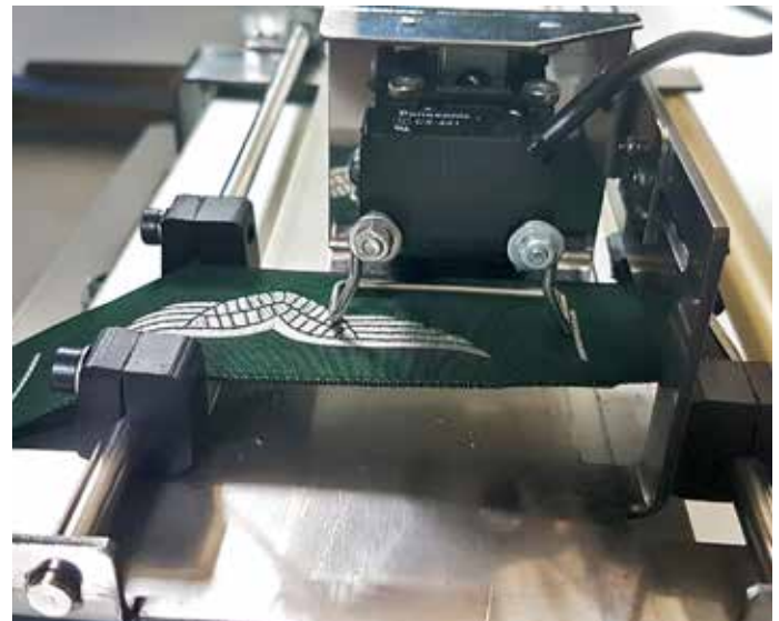
ROLL2BASKET SENSOR FOR TAPES FOR ROLL2BASKET Potential applications are ribbons with textile printing or weaving that have a defined area where embroidery needs to be placed on point.
