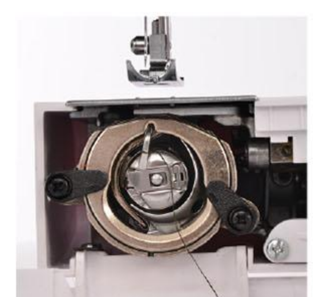
Industrial vertical swing shuttle
