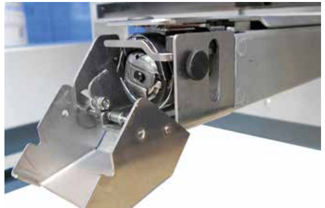
The standard tubular arm offers a protective flap, that no material will get caught by the picker.
