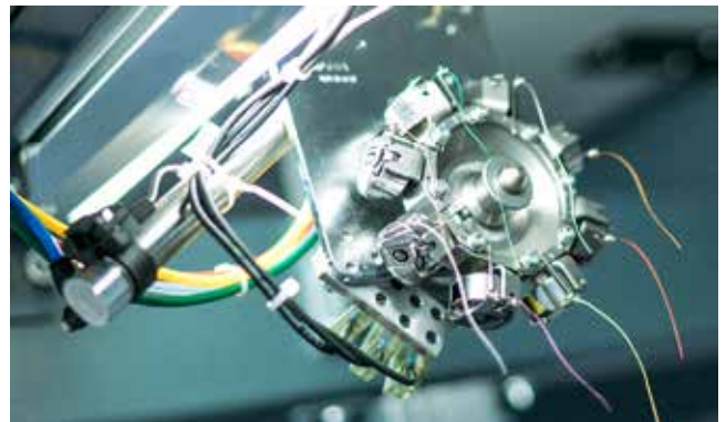
Optional Auto Select Bobbin Changer- Software-controlled use of the appropriate bobbin thread; e.g. by colour, conductivity or material.
