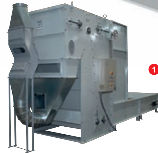
BALES MIXER-OPENER AB
