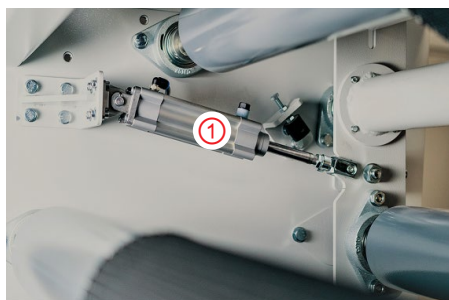
Pneumatic swing-mechanism
