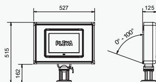
Protective cabinet with 12 inch HMI and rotating base
