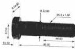
YSM VOL 81 VOLVO HUB BOLT OEM NO. 3302107800
