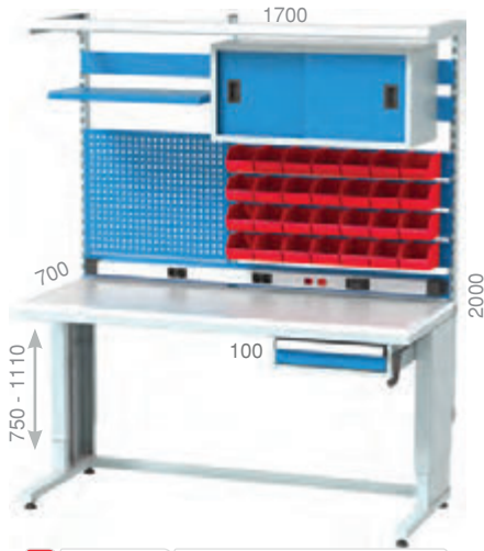
3634 1700 X 700 X 2000 mm 1 Adet / Pieces A-150 125 X 190 X 98 mm 28 Adet / Pieces
