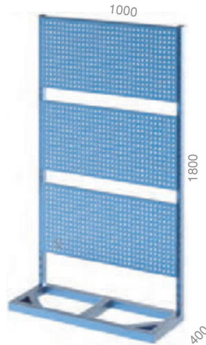
4550 1000 X 400 X 1800 mm
