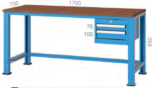
3310 1700 X 700 X 850 mm 2 Adet / Pieces
