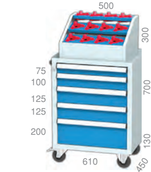
2245 610 X 450 X 1130 mm 12 Adet / Pieces 1 Adet / Pieces
