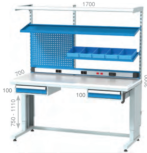
3627 1700 X 700 X 2000 mm 2 Adet / Pieces A-100 102 X 170 X 74 mm 14 Adet / Pieces
