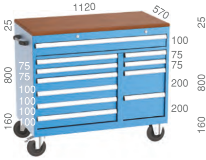
8330 1120 X 570 X 985 mm 11 Adet / Pieces
