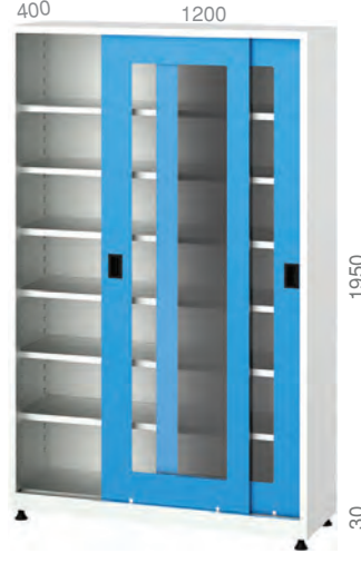
> 6560 1200 X 400 X 1980 mm
