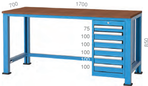
3131 1700 X 700 X 850 mm 6 Adet / Pieces
