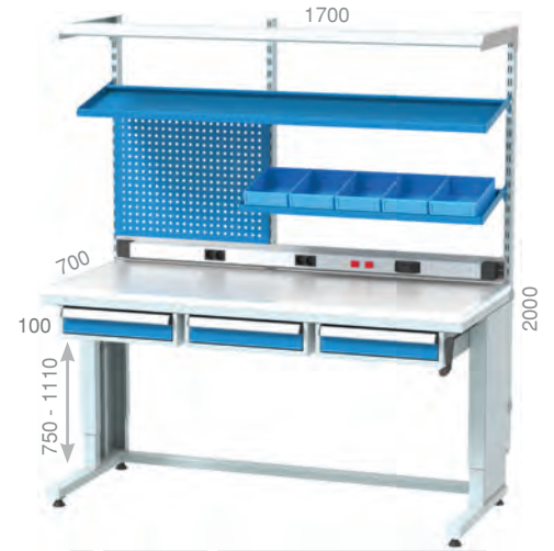
3628 1700 X 700 X 2000 mm 3 Adet / Pieces A-100 102 X 170 X 74 mm 14 Adet / Pieces
