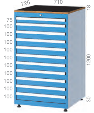
7201 710 X 725 X 1248 mm 11 Adet / Pieces
