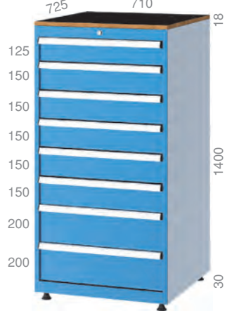
7402 710 X 725 X 1448 mm 8 Adet / Pieces
