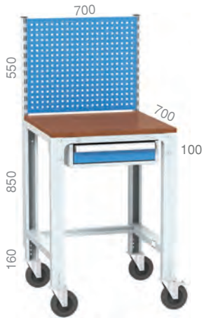
➤ 3381 700 X 700 X 1560 mm
