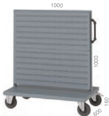
> 7620 1000 X 1000 X 1160 mm
