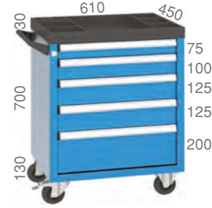
8075 610 X 450 X 860 mm 5 Adet / Pieces
