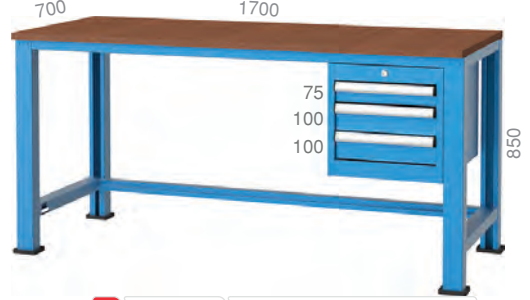
3110 1700 X 700 X 850 mm 3 Adet / Pieces
