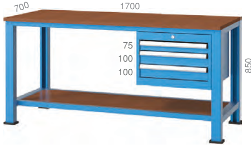
3710 1700 X 700 X 850 mm 3 Adet / Pieces
