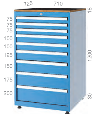
7200 710 X 725 X 1248 mm 9 Adet / Pieces
