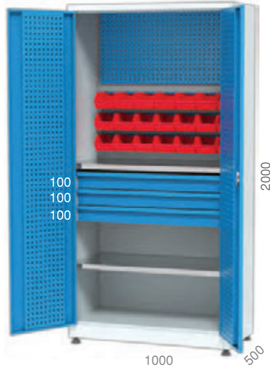
6381 1000 X 500 X 2000 mm A-150 21 Adet / Pieces 3 Adet / Pieces
