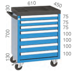
8077 610 X 450 X 860 mm 7 Adet / Pieces
