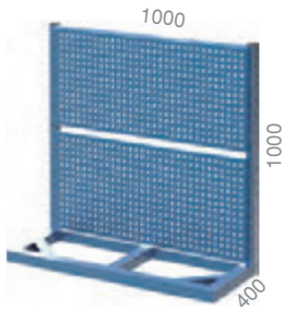
4555 1000 X 400 X 1000 mm
