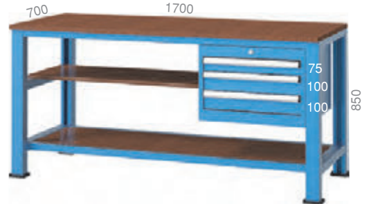
3730 1700 X 700 X 850 mm
