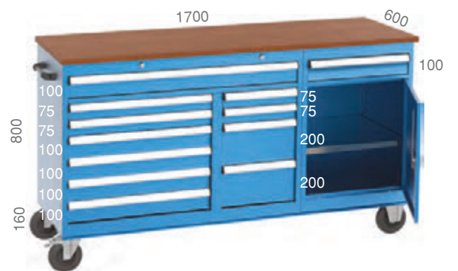
➤ 8415 1700 X 600 X 985 mm
