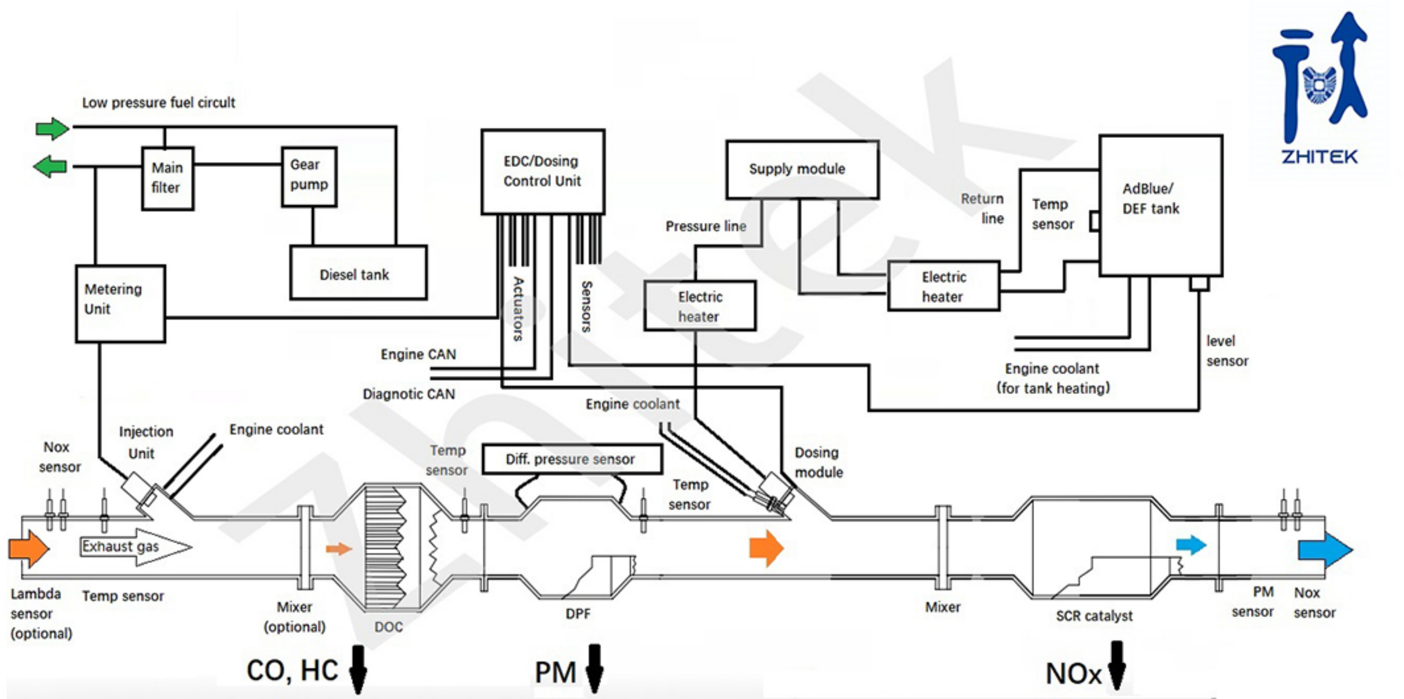
Schematic diagram of a diesel vehicle aftertreatment system
