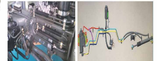
翅片散热管的应用 Application of fin heat pipe
