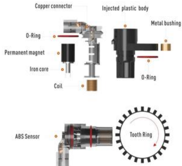
Passive ABS sensor (Magnetolectric ABS sensor)
