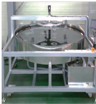
Durability Tester
