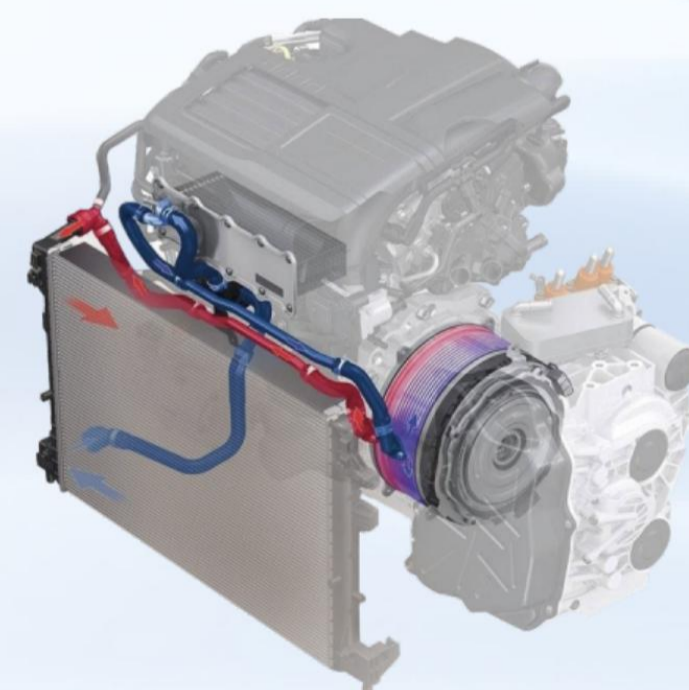
散热器/Radiator
