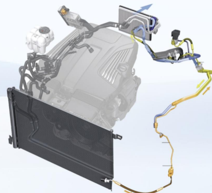
冷凝器/Condenser
