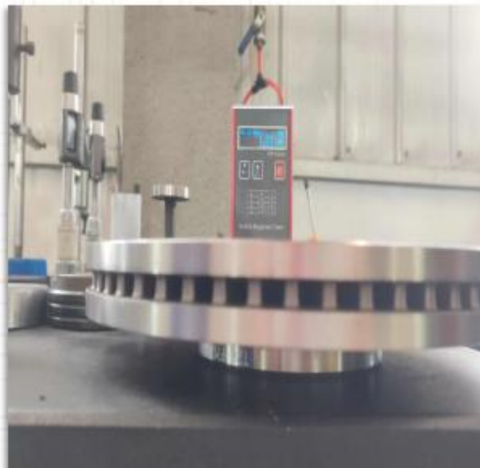
粗糙度检具 Roughness gauge
