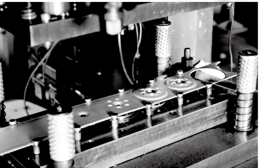
REINFORCED PLATE PRESS LINE
