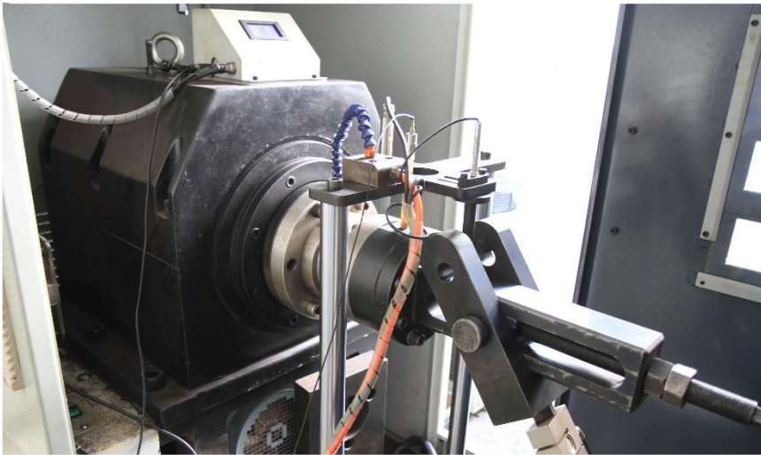
Wheel hub bearing dynamic no-load torque testing machine
