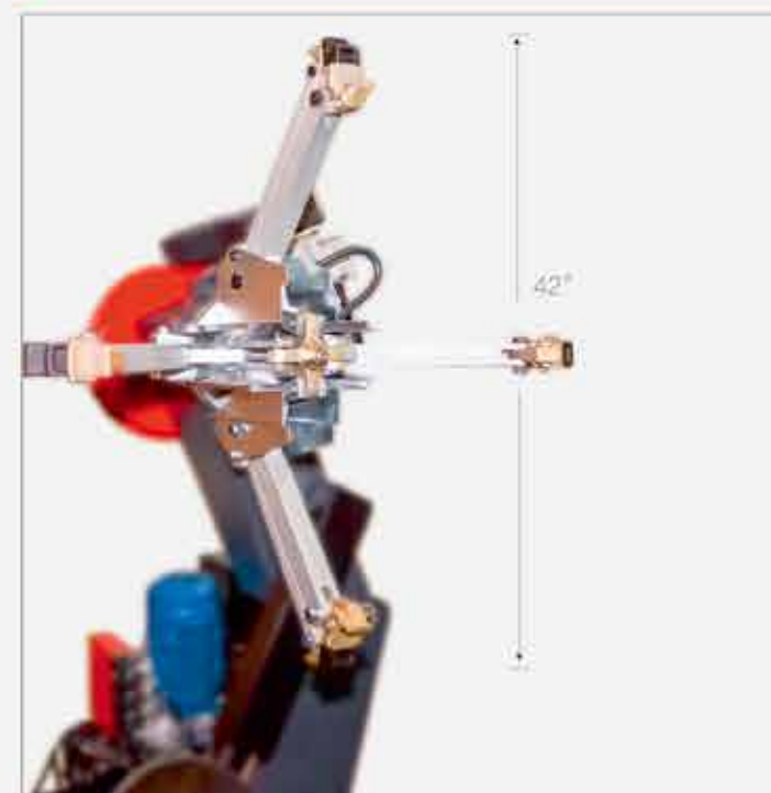
通用自动定心卡盘，操作尺寸从14" 到42" UNIVERSAL SELF-CENTRING CHUCK, OPERATE SIZE FROM 14" TO 42"
