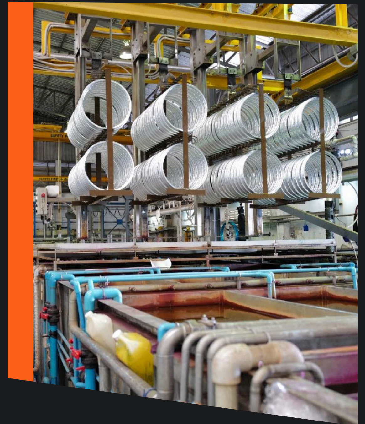
ANODIZATION AUTO LINE
