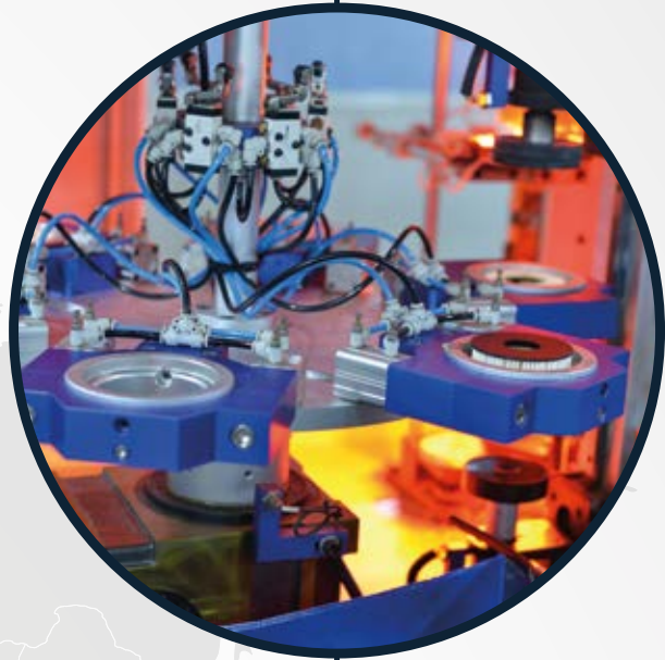
HOT BONDING
