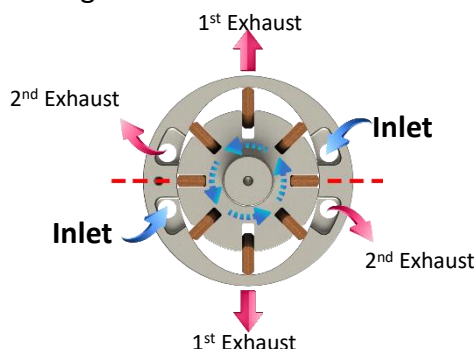
Double Air Intake
