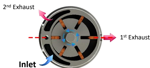
Air-Intake Normal Type
