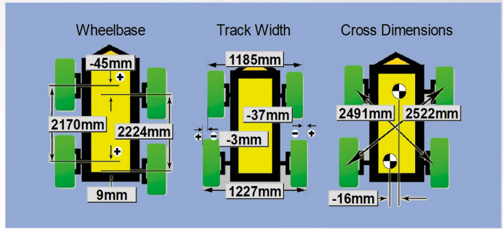
Cross Chassis Measurement
