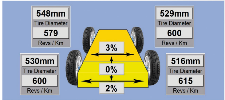
Measurement of Wheel Diameter and Number of Laps Per Kilometer
