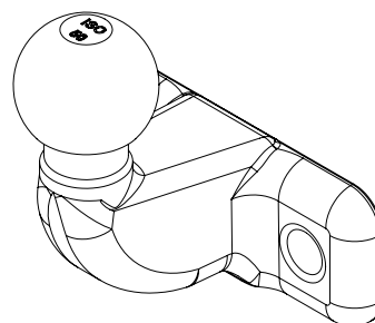
Ball type B
