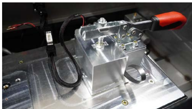
Equipment for testing and diagnostics of valve bodies and solenoids of automatic transmissions
