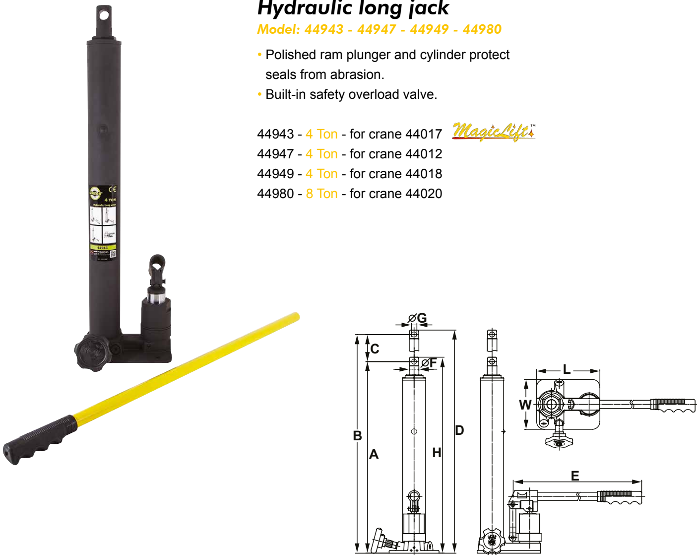
HYDRAULIC LONG JACK
