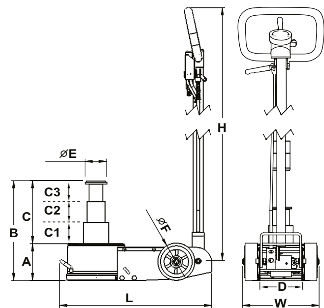
AIR OPERATED AXLE JACKS
