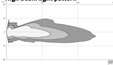
Low beam light pattern
