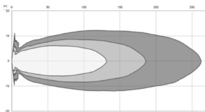
High beam light pattern
