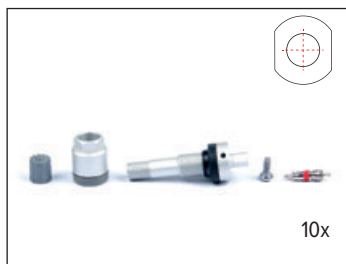
Clamp-in Italsensor
