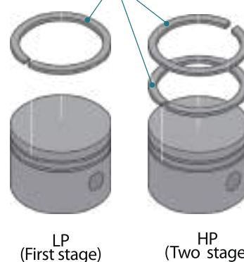
Pressure ring
