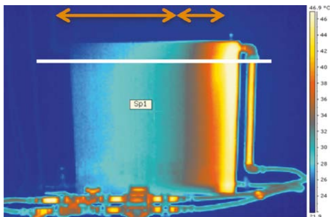
Air effect on radiator power output (*)
