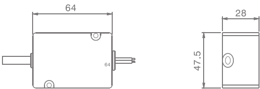
Dimensions (mm)
