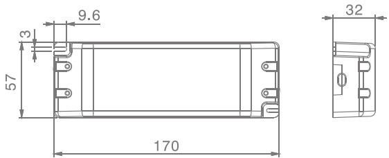
Dimensions (mm)
