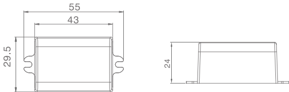
Dimensions (mm)
