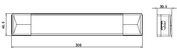
Dimensions (mm)
