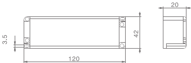
Dimensions (mm)
