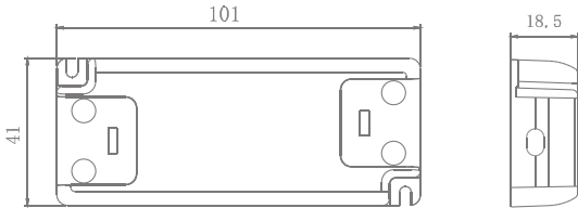
Dimensions (mm)
