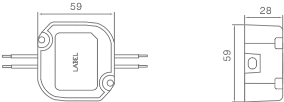
Dimensions (mm)
