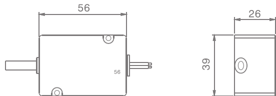
Dimensions (mm)
