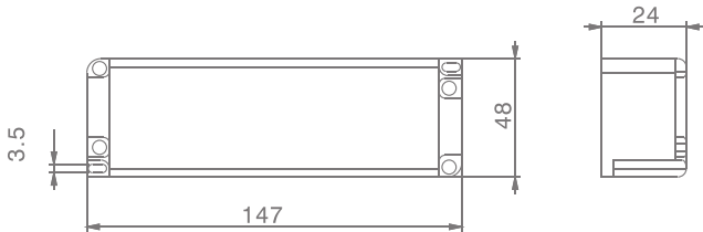
Dimensions (mm)
