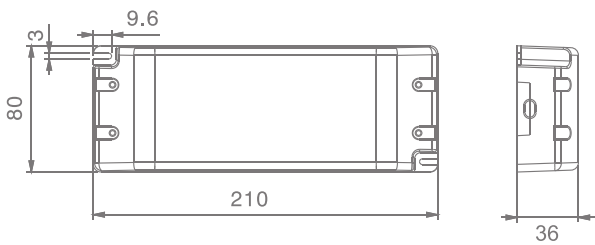
Dimensions (mm)
