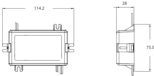
Dimensions (mm)
