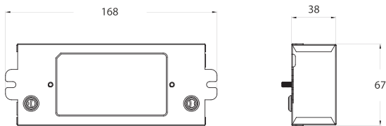
Dimensions (mm)
