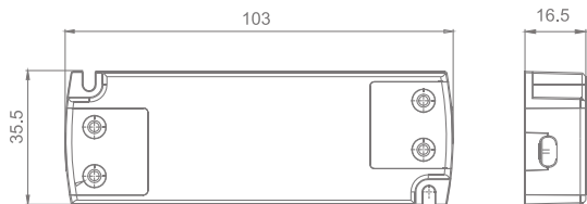
Dimensions (mm)
