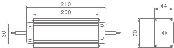
Dimensions (mm)
