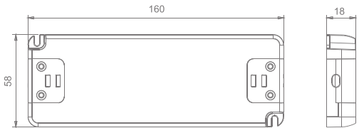
Dimensions (mm)
