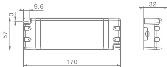
Dimensions (mm)
