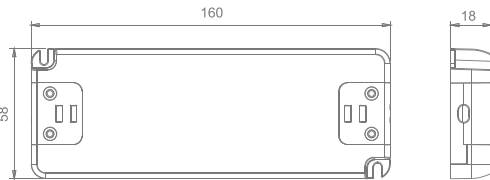
Dimensions (mm)
