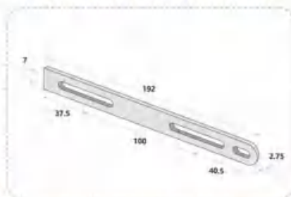
TFM Adjustable Connector
