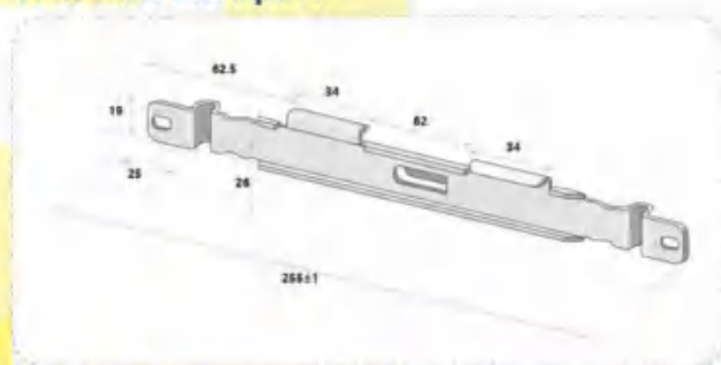
TFM Fast Fix Splice
