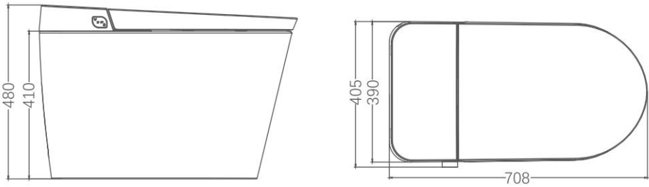
Dimension: 708x405x480mm
