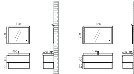
SV1200WH01/S18 Veneer & Painting
