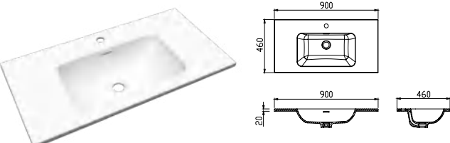
Matte White Solid Surface Basin
