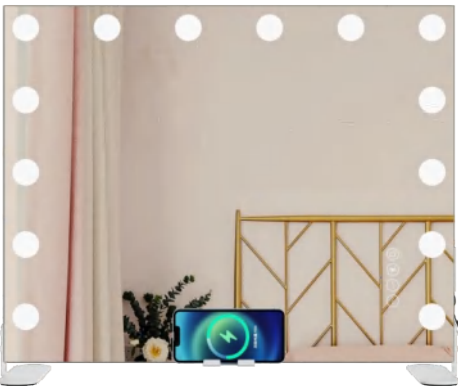
DP357S NEW PRODUCT BT speaker + wireless charging 蓝牙音响+无线充功能 产品尺寸/Size: W58*H46cm, W22.8"*H18" 材质/Material: Iron frame & base + MDF backboard 铁框&底座+MDF背板
