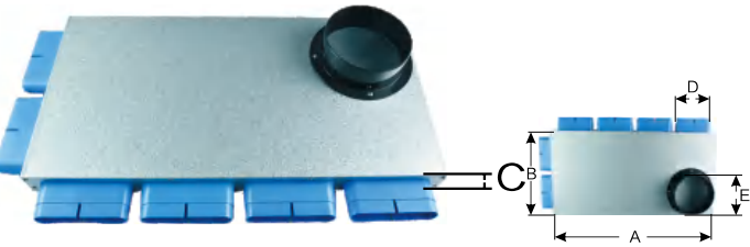
Floor Supply Air branch 1 divide 6
