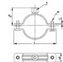
SCP-E Pipe Clamp with Hex Nut
