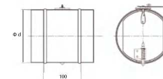
RDD Regulating Damper
