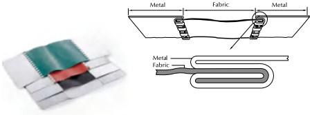
FCN Flexible Duct Connector
