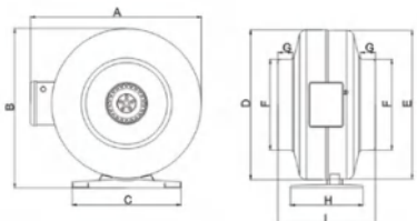
FZY Installation dimension sheet
