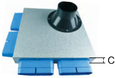
Floor Supply Air branch 1 divide 4
