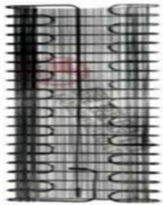
Wire on Tube Condenser with C-bending
