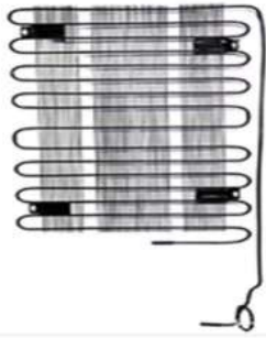
Wire on Tube Condenser with Mounting Clamp
