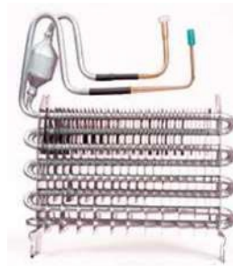
Continuous Fin Type FF Evaporator
